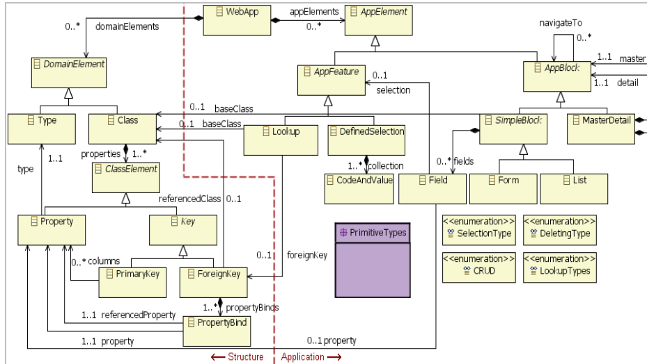
Fig. 2. Diagram of the Web Application Metamodel. Here all the elements of the metamodel are shown.
